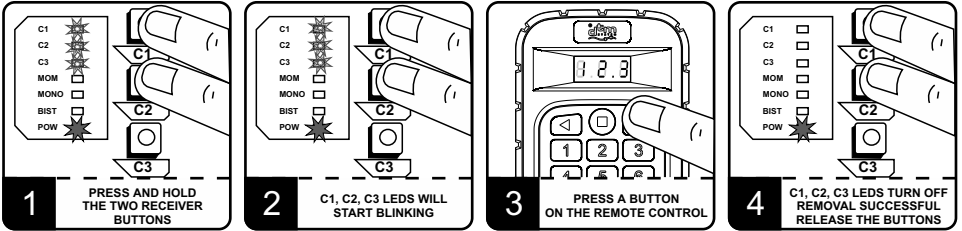
Fig. 4 Removing the transmitter.
